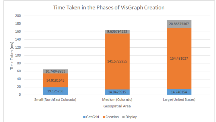
Figure 6 – The time taken during various phases of GeoLens.
