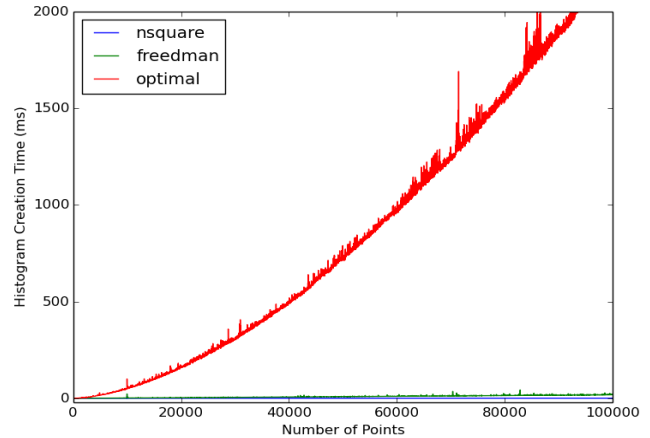
Figure 5. The creation time of the three different methods. Even with only 5000 points, the scalability of the optimal histogram generation comes into question, but the other two methods scale.
